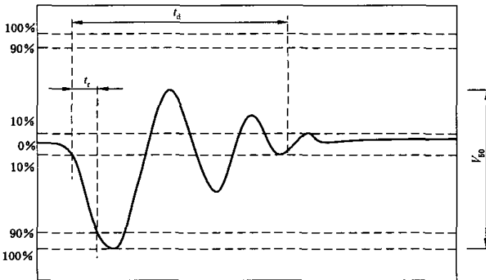
c) 谐波脉冲
