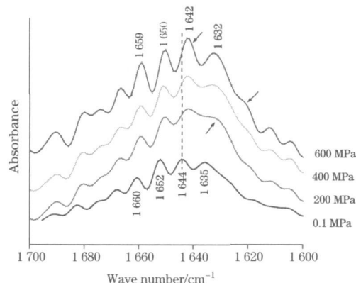
Fig. 2 Stacked plots of deconvoluted FTIR spectra of untreated and HP-treated ( 200 \sim 600 \text{ MPa} ) SPI. The arrows indicate the observable changes in the intensity or wave-number shift of the corresponding bands
