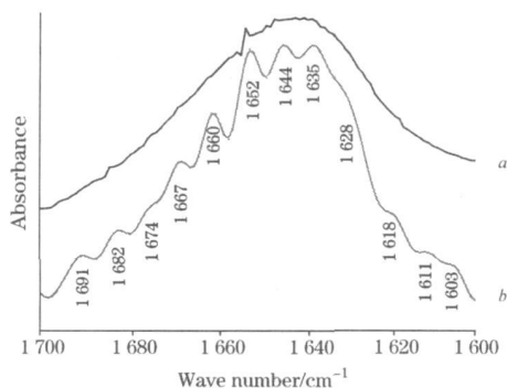
Fig 1 A typical FTIR spectrum of 10 \text{ g} \cdot (100 \text{ mL})^{-1} SPI
