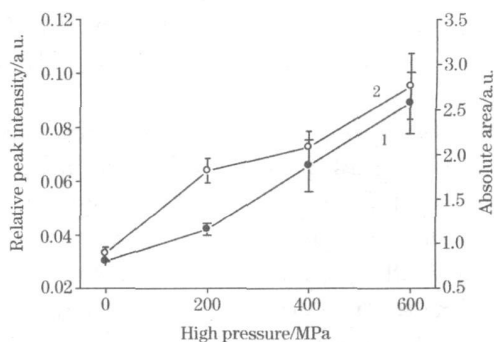
Fig 5 Effects of HP treatment on the peak intensity of the band at 1507\text{ cm}^{-1} (relative to the baseline) and absolute area of amide II bands of SPI
