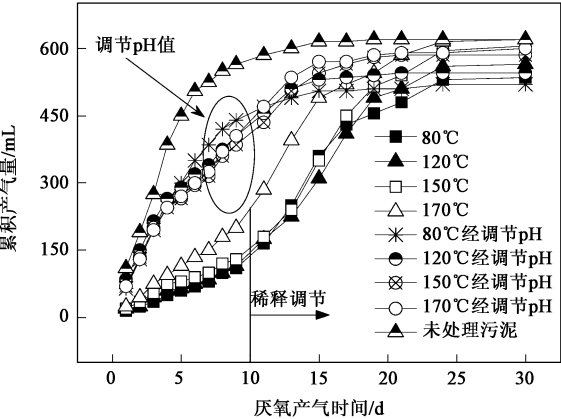
图 8 污泥累积产气量[ m(\text{NaOH})/m(\text{SS}) = 0.1 ] Fig. 8 Biogas production [ m(\text{NaOH})/m(\text{SS}) = 0.1 ]
