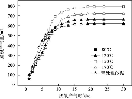
图 7 污泥累积产气量[ m(\text{NaOH})/m(\text{SS}) = 0.05 ] Fig. 7 Biogas production [ m(\text{NaOH})/m(\text{SS}) = 0.05 ]
