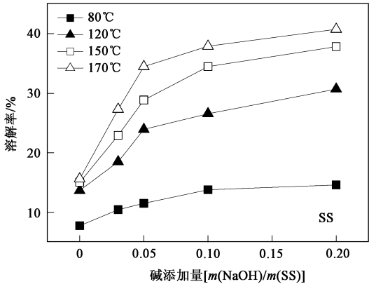
图 6 不同碱添加量下的固体溶解规律 Fig. 6 Solid dissolving trend at different alkali addition dose
