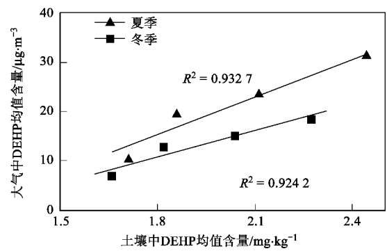
图2 采样点大气与土壤中 DEHP 含量的相关性 Fig.2 Relationship of DEHP between air and agriculture soil
