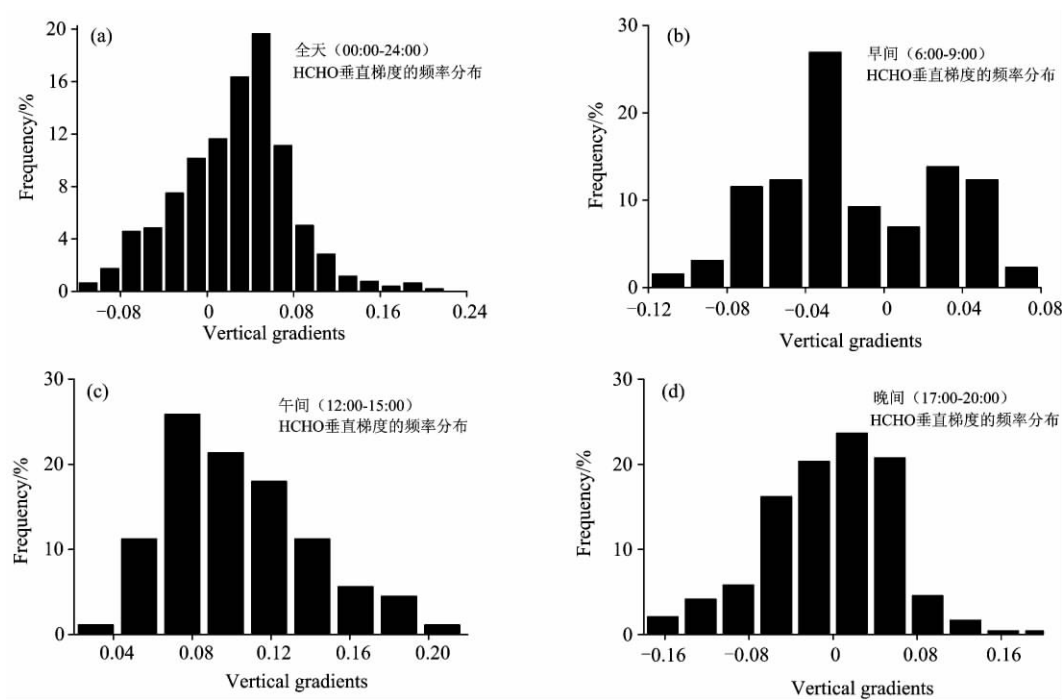
Fig 5 Vertical distribution frequency characteristics of HCHO
