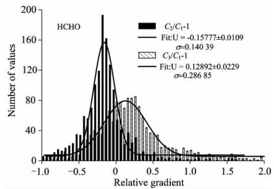
Fig 7 Gauss distribution of the relative gradients of HCHO
