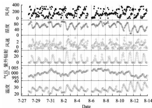
Fig 3 Time series of meteorological data
