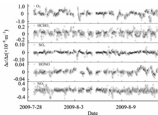
Fig 4 Time series of the vertical gradient
