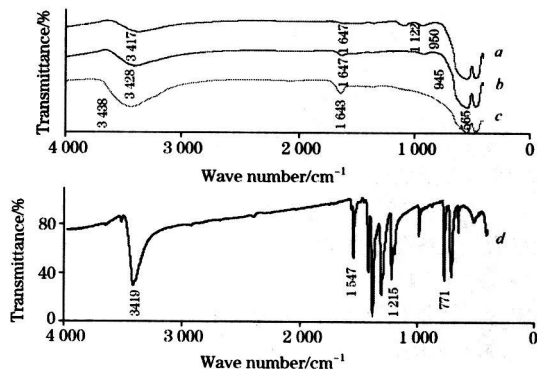
Fig. 3 Variation of IR spectra of hematite after PCP adsorption at different pH
