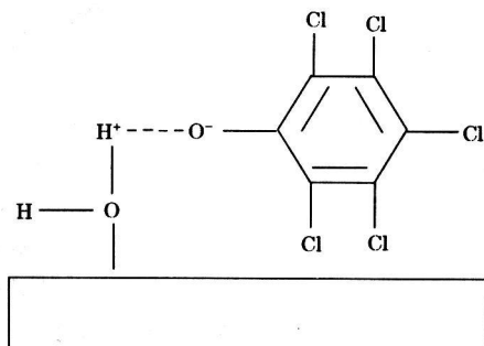
Fig. 4 Schematic diagram of adsorption of PCP on hematite at pH 6.0
