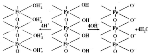
Fig 2 Schematic diagram of formation of \alpha\text{-Fe}_2\text{O}_3 surface and surface charge
