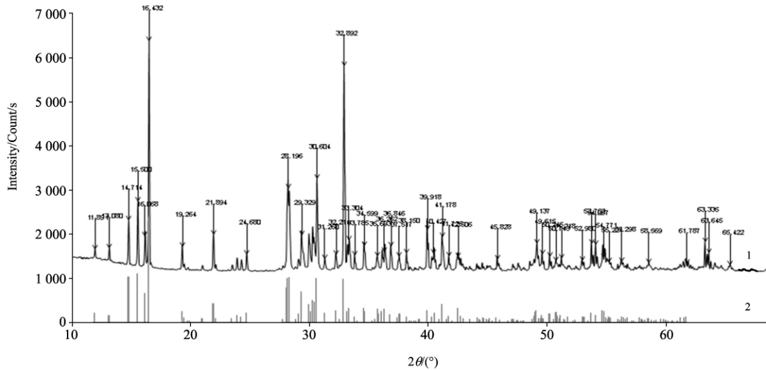
(a) File: 31 10-06-04. raw-Type: 2Th/Th locked-Start: 10. -End: 70-Step: 0.020 -Step time: 11.2 s-Temp.: 27-Time Started: 6 s-2-Theta (b): 01-071-2434(C)-Realgar-AsS-Y: 37.22%-dx by: 1.-WL: 1.540 6-Monoclinic-a 9.325 00-b 13.571 00-c 6.587 00-alpha 90.000 -beta-106.380-gamma 90.000-Primitive-P2 1 /n(14)-16-799.749-I/I 0 : PDF 1.6-
