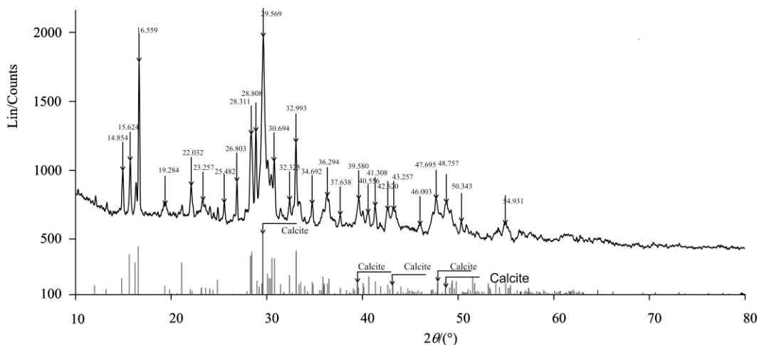
☒ File: 1003-25.raw-Type:2Th/Th locked-Start:10.0-End:80.0-Step:0.020-Step time:16.8s-Temp:24-Time Started: 6s-2-Theta: 10.0-Theta: 5.0 ☒ 01-073-2112 (C)- Realgar - As 4 S 4 - Y: 18.35 %- d x by: 1.- WL: 1.5406- Monoclinic- a 9.27000 - b 13.50000- c 6.56000- alpha 90.000- beta 106.620- gamma 90.000- Primitive- P21/n (14) -16 -786.654- I/Ic PDF 0.9- ☒ 01-072-1650 (C)- Calcite- CaCO 3 - Y: 25.00 %- d x by: 1.- WL: 1.5406- Rhombo.H.axes- a 4.99300- b 4.99300- c 16.91700- alpha 90.000- beta 90.000- gamma 120.000-Primitive- R-3c (167)- 6- 365.239- I/Ic PDF
