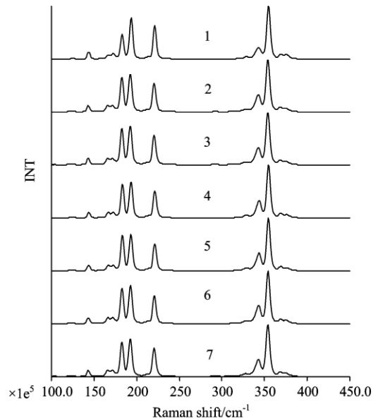
Fig 9 Raman spectra of prepared realgar with different processing procedures
