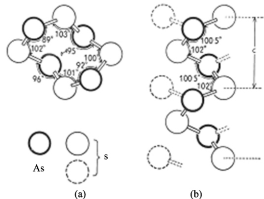
Fig 10 Molecular structures of (a): realgar and (b): orpiment. In (b) is shown an As 2 S 2 spiral chain (heavy and light full circles), and an As 2 S 3 layer (full and broken circles). Reproduced from Ito, Morimoto and Sadanaga, 1952)
