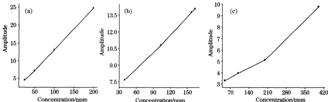
Fig 2 (a) : The relation between the value of the characteristic frequency and the concentration in the SO 2 frequency drawing of Fourier transformation in 280-310 nm; (b) : The relation between the value of the characteristic frequency and the concentration in the NO frequency drawing in 200-220 nm; (c) : The relation between the value of the characteristic frequency and the concentration in the NO 2 frequency drawing in 420-450 nm
