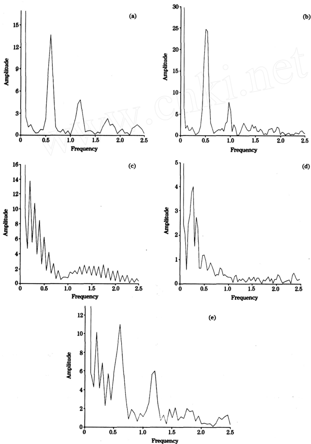
Fig 1 (a) : The frequency drawing of Fourier transformation of SO 2 absorption spectrum in 200-220 nm (b) : The frequency drawing of SO 2 in 280-310 nm; (c) : The frequency drawing of NO in 200-220 nm; (d) : The frequency drawing of NO 2 in 420-450 nm; (e) : The frequency drawing of SO 2 and NO in 200-220 nm
