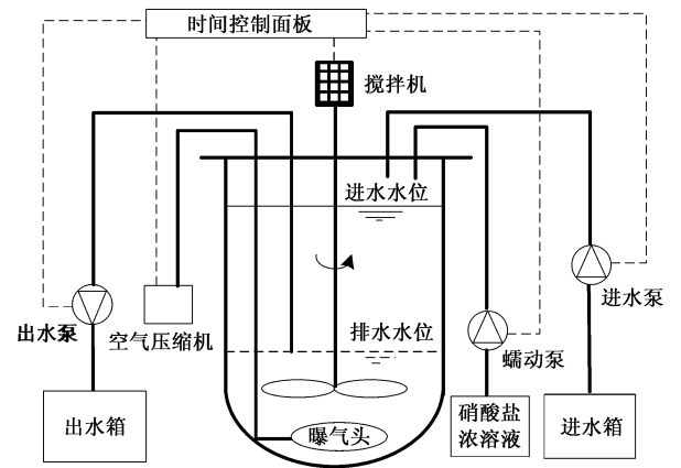
图 1 SBR 示意 Fig.1 Schematic diagram of the SBR used in this study
