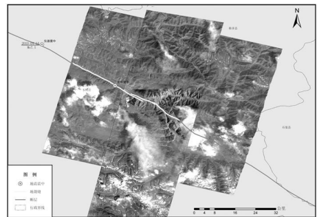
Fig 9 Distribution of ground fissure
