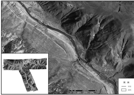
Fig 11 Distribution of earthquake subsidences
