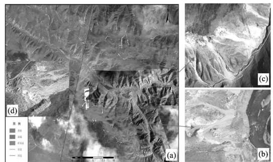
Fig 10 Distribution of Landslides, collapses and debris flows
