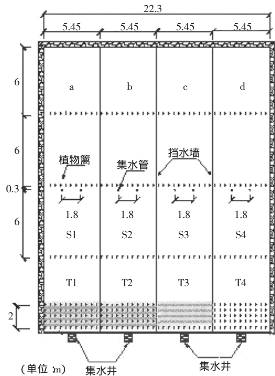
图 1 供试坡地的平面设计图 Figure 1 Plan view of the sloping
