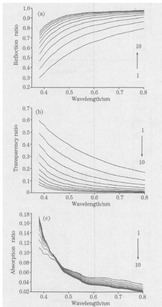
Fig 5 Reflection ratio, transparency ratio and absorption ratio of different thickness of silver films
