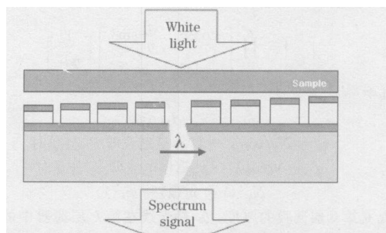
Fig. 1 Basic structure of the miniature Fabry-Perot spectrum instrument
