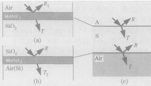
Fig 3 Equivalent predigestion of optical configuration
