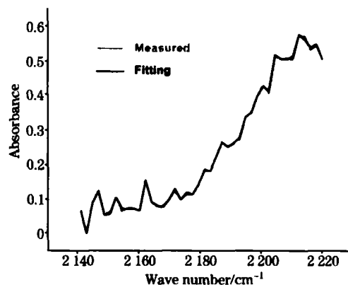
Fig 5 Measured spectrum and fitting spectrum of \text{CO} and \text{N}_2\text{O}
