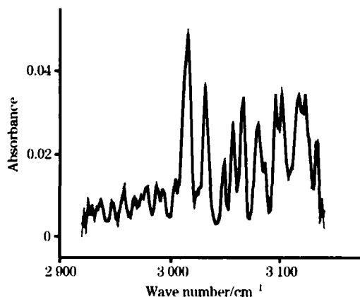
Fig 2 Measured spectrum and fitting spectrum of \text{CH}_4
