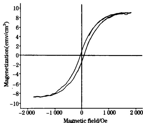
Fig 3 Magnetization hysteresis loops for Ni-doped ZnO film with Ni content of 5 mol % at 300 K
