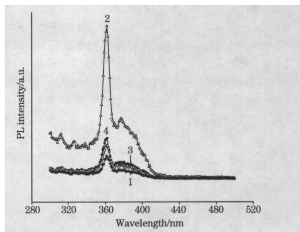
Fig 5 Fluorescence emission spectra of Ni-doped ZnO films with different Ni contents (R T= 0.5 Pa) 1: 0.07; 2: 0.05; 3: 0.03; 4: 0.01
