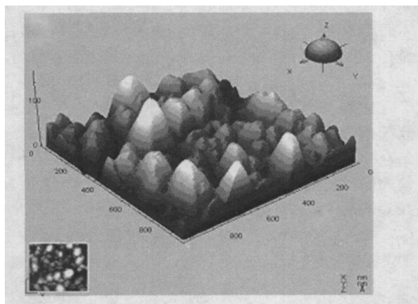
Fig 2 AFM image of ZnO: Ni film prepared by target with Ni concentration of 5 mol%
