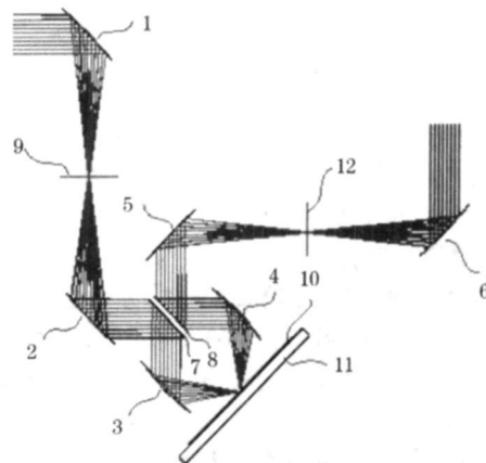
Fig. 3 Layout of the detecting optical path
