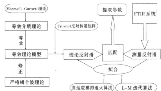
Fig 1 FTIR measurement system flowchart
