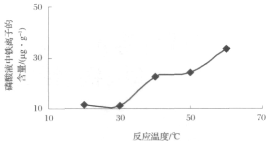
图 3 反应温度对除铁效果的影响 Figure 3. Effects of temperature on iron removal efficiency.
