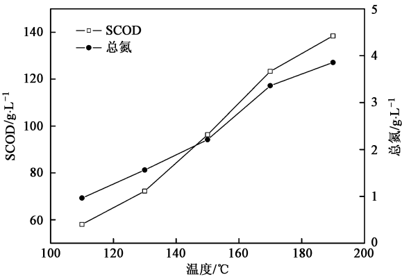
图1 预处理后SCOD和总氮随温度变化 Fig. 1 Changes of SCOD and TN after pretreatment at different temperature
