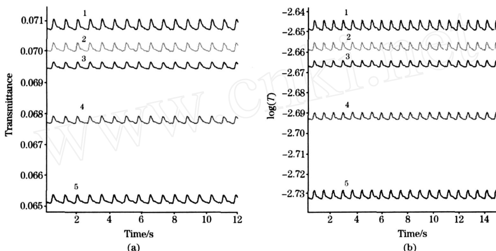
Fig 1 Photoelectric pulse wave (a) and the logarithm pulse wave (b) 1: 1 110 nm; 2: 1 115 nm; 3: 1 120 nm; 4: 1 125 nm; 5: 1 130 nm
