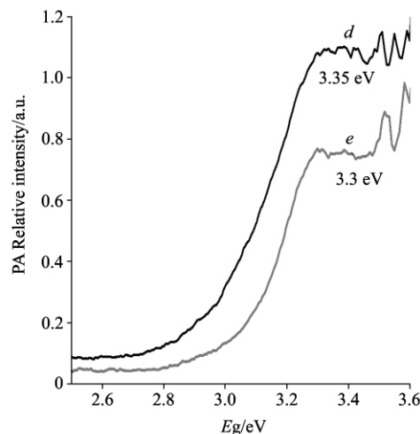
Fig 7 Al-doped ZnO and ZnO semiconductor nano-crystalline powder photoacoustic spectra
