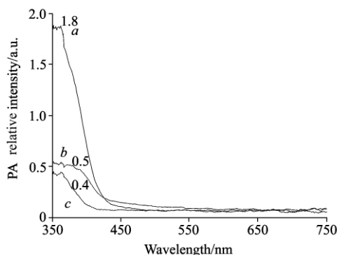
Fig 4 Three different particle size of \text{TiO}_2 semiconductor nano-crystalline powder photoacoustic spectra
