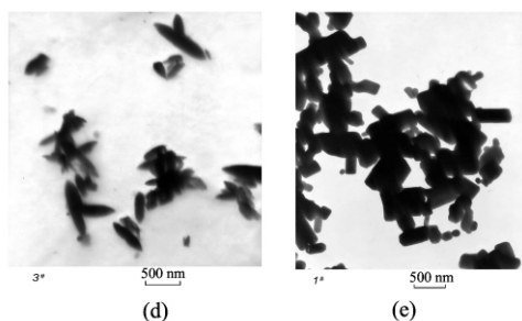
Fig 3 Al-doped ZnO and ZnO semiconductor nano-crystalline powder TEM image
