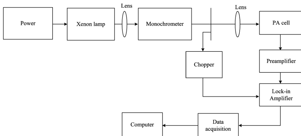
Fig 1 Diagram of experimental setup for measurements of photoacoustic spectroscopy
