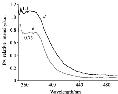
Fig 6 Al-doped ZnO and ZnO semiconductor nano-crystalline powder photoacoustic spectra
