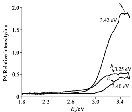
Fig 5 Three different particle size of \text{TiO}_2 semiconductor nano-crystalline powder photoacoustic spectra
