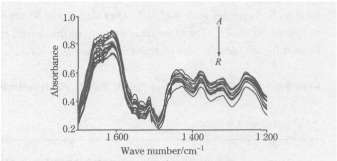
Fig 2 FTIR spectra of epimedium koreanum nakai from different producing area
