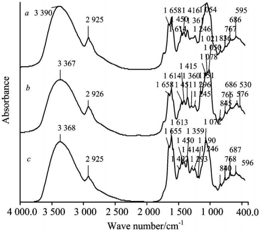
Fig 1 FTIR spectra of a wine fried scutellariae, b sliced scutellariae and c crude drug of radix scutellariae
