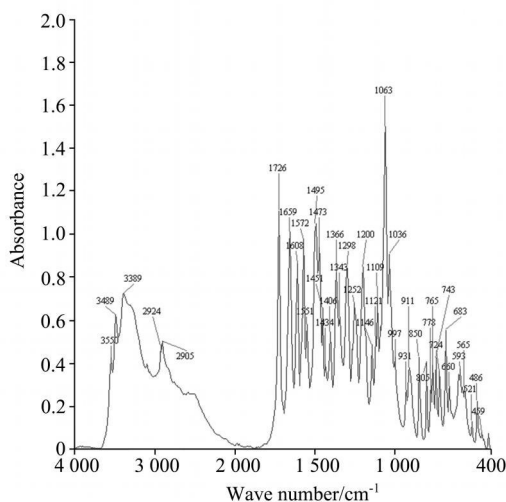
Fig 4 Molecule structure and FTIR spectra of baicalin
