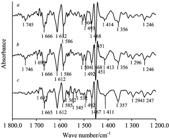
Fig 2 Second derivative spectra of a wine fried scutellariae, b sliced scutellariae and c crude drug of radix scutellariae
