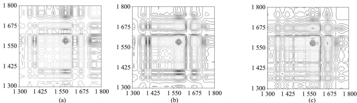
Fig 3 Two dimensional infrared (2D IR) correlation spectroscopy of (a) wine fried scutellariae, (b) sliced scutellariae and (c) crude drug of radix scutellariae
