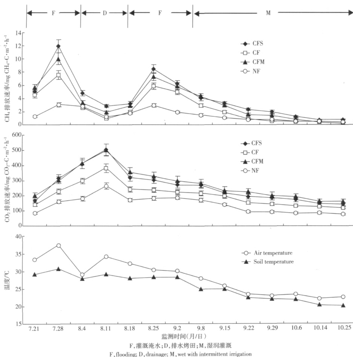
图 1 水稻生长期间 \text{CH}_4 和 \text{CO}_2 排放及土壤温度(5 cm)和气温的变化动态 Figure 1 Dynamics of \text{CH}_4 and \text{CO}_2 emissions, air and soil temperature during rice growing
