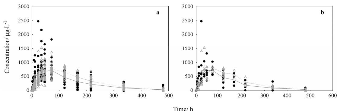
Figure 2 Plasma concentration-time plot of dense data (a) and sparse data (b). The black points represent the observed concentration of healthy subjects, the grey points represent the observed concentration of patients, the solid line represents the mean concentration-time curve of healthy subjects, and the dotted line represents the mean concentration-time curve of patients
