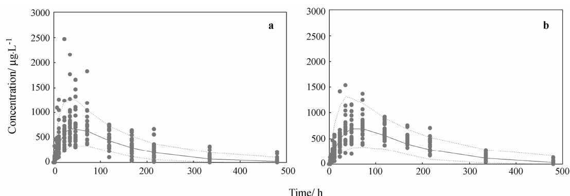
Figure 4 A visual assessment of the posterior predictive performance of the final model in terms of its ability to predict the observed dense data. Healthy (a) and patients (b) concentration-time profile of drug A. The lines represent the 5th, 50th and 95th percentiles of concentration distribution in each panel
