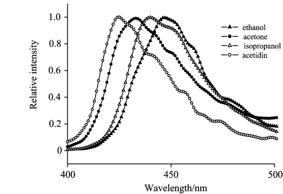
Fig 2 Fluorescence emission spectrum in different solvent
