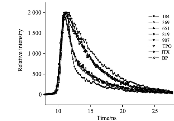
Fig 1 Transient fluorescence spectra of different photoinitiator
