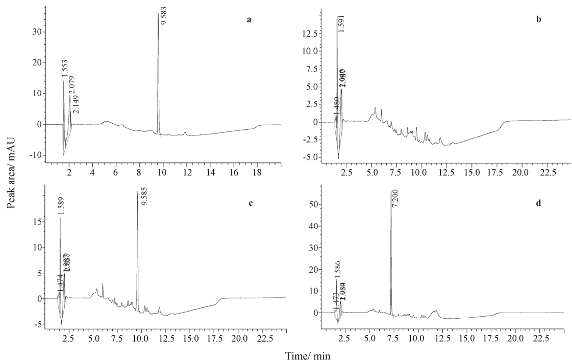
Figure 5 HPLC chromatograms of clopidogrel bisulfate and its carboxylic acid metabolite. a: Clopidogrel ( 10\text{ }\mu\text{g}\cdot\text{mL}^{-1} ); b: Plasma; c: Plasma spiked with clopidogrel ( 10\text{ }\mu\text{g}\cdot\text{mL}^{-1} ); d: Plasma after clopidogrel bisulfate administration
