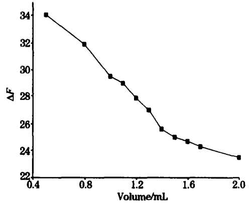
Fig 3 Effect of amount of H 2 SO 4
