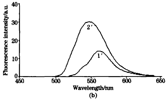
Fig 1 Excitation spectrum (a) and emission spectrum (b) 1, 1': AR+ H 2 SO 4 ; 2, 2': Cr( VI) + AR+ H 2 SO 4
