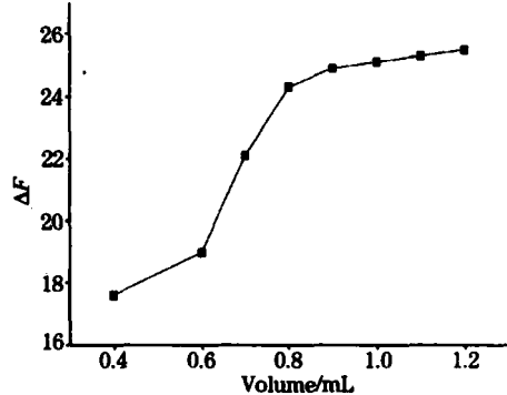
Fig 5 Effect of amount of acridine red
