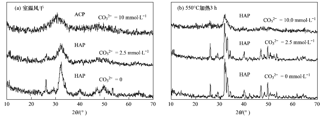
图 5 pH=9.0 时不同 \text{CO}_3^{2-} 浓度下沉淀产物室温风干及其 550℃加热 3 h 后的 XRD 谱图 Fig.5 XRD spectra of precipitation product dried at room temperature and heated for 3 hours at 550℃ under different \text{CO}_3^{2-} concentrations at pH=9.0
