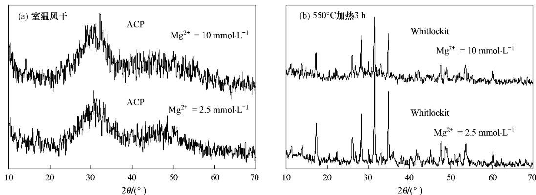
图 7 \text{pH} = 9.0 时不同 \text{Mg}^{2+} 浓度下沉淀产物室温风干及其 550^\circ\text{C} 加热 3 h 后的 XRD 谱图 Fig. 7 XRD spectra of precipitation product dried at room temperature and heated for 3 hours at 550^\circ\text{C} under different \text{Mg}^{2+} concentrations at \text{pH} = 9.0
