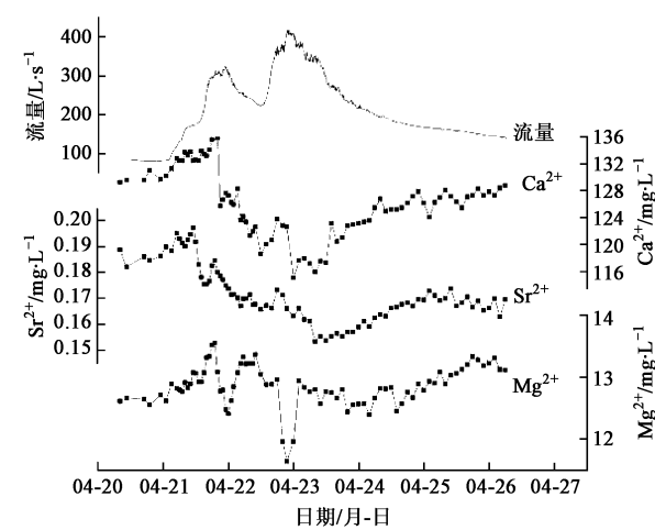
图6 2008年4月下旬姜家泉中与碳酸盐岩溶解有关的阳离子浓度变化趋势 Fig. 6 Concentrations variation of carbonate-derived dissolution cations at Jiangjia Spring in late April 2008
