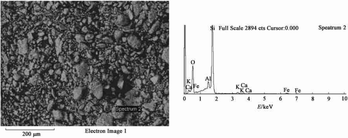
图5 c阶段姜家泉泉水中悬浮颗粒物(大颗粒)SEM和EDS图 Fig. 5 SEM micrograph and EDS of the large size particle SPM during the c phase at Jiangjia Spring
