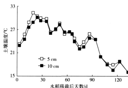
图 3 土壤温度的季节变化 Figure 3 Seasonal variation of soil temperature
