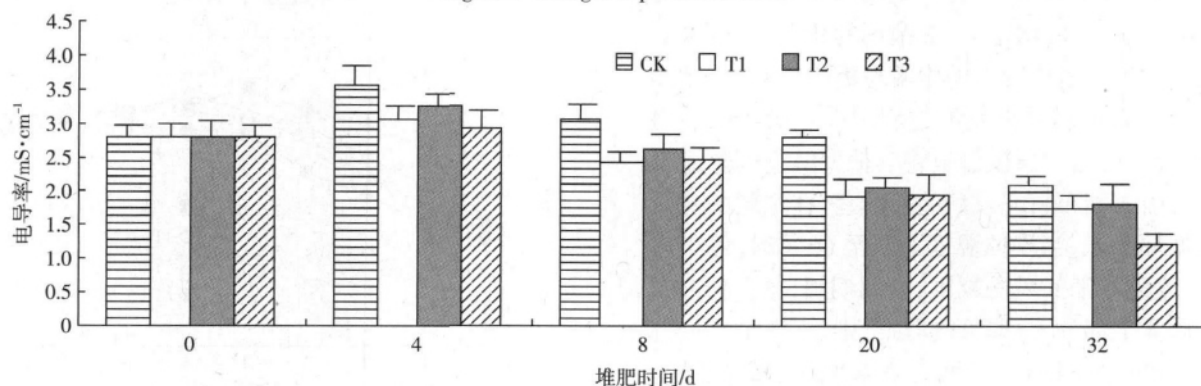
图 3 堆肥过程中电导率的变化 Figure 3 Changes of electrical conductivity of four trials
