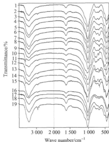
Fig 1 Infrared spectra of Lapis Micae Aureum samples
