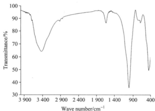
Fig 2 Reference infrared spectra of Lap is Micae Aureum
