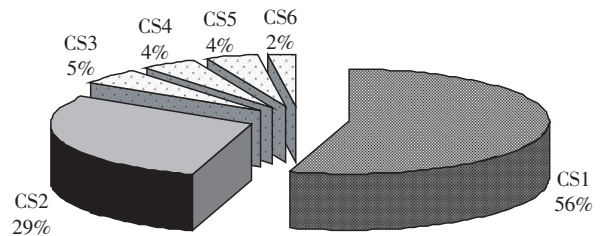
图 3 复合菌群 JZ-1 的 16S rDNA Rsa 酶酶切 OTU 及所在比例 Figure 3 OTU and its percentage of microbial community JZ-1 amplified 16S rDNA after digestion by Rsa
