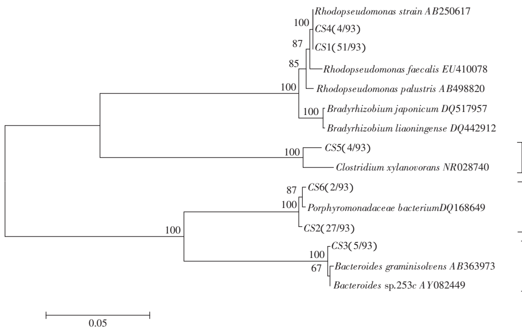
The number at each branch points is the percentage supported by bootstrap. Bar 5% sequence divergence. Numbers in brackets indicate the clone number out of total clones.
