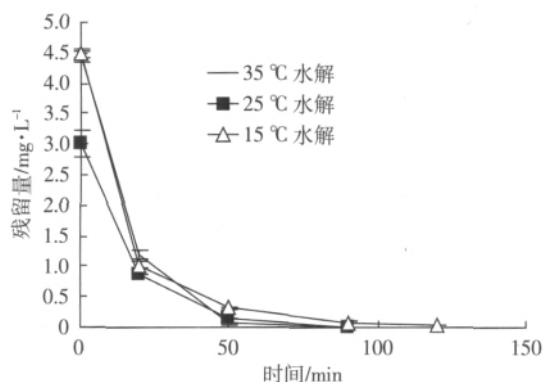
图 1 不同温度下 2,4-D 丁酯在 pH 9 缓冲液中的水解曲线 Figure 1 Hydrolytic curves of 2,4-D butylate in buffer solution of pH 9 at the different temperatures
