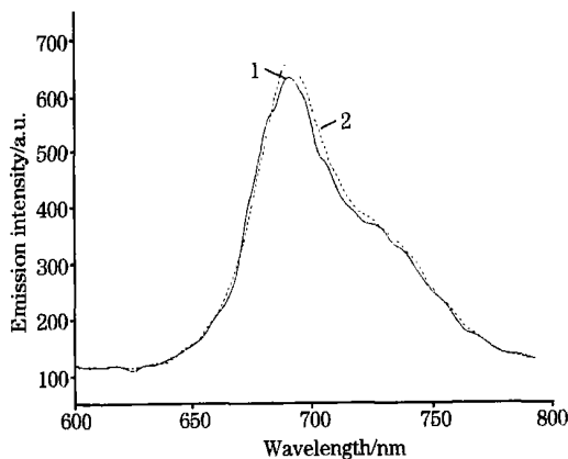
Fig. 1 The fluorescence spectrum and delayed fluorescence spectrum of isolated chloroplasts: Excited by blue light (438 nm), slits: Ex = Em = 10 nm, at PHOS model, gate time: 10 ms, delay time for delayed fluorescence spectrum is 1 000 ms, cycle time: 1 020 ms. \log_2 c = 2 ( 7.8 \mu\text{g mL}^{-1} ), c : Concentration
