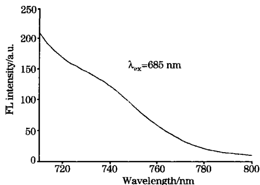
Fig. 5 The fluorescence emission spectrum of spinach chloroplasts, excited by 685 nm, Ex = 5 nm, Em = 10 nm
