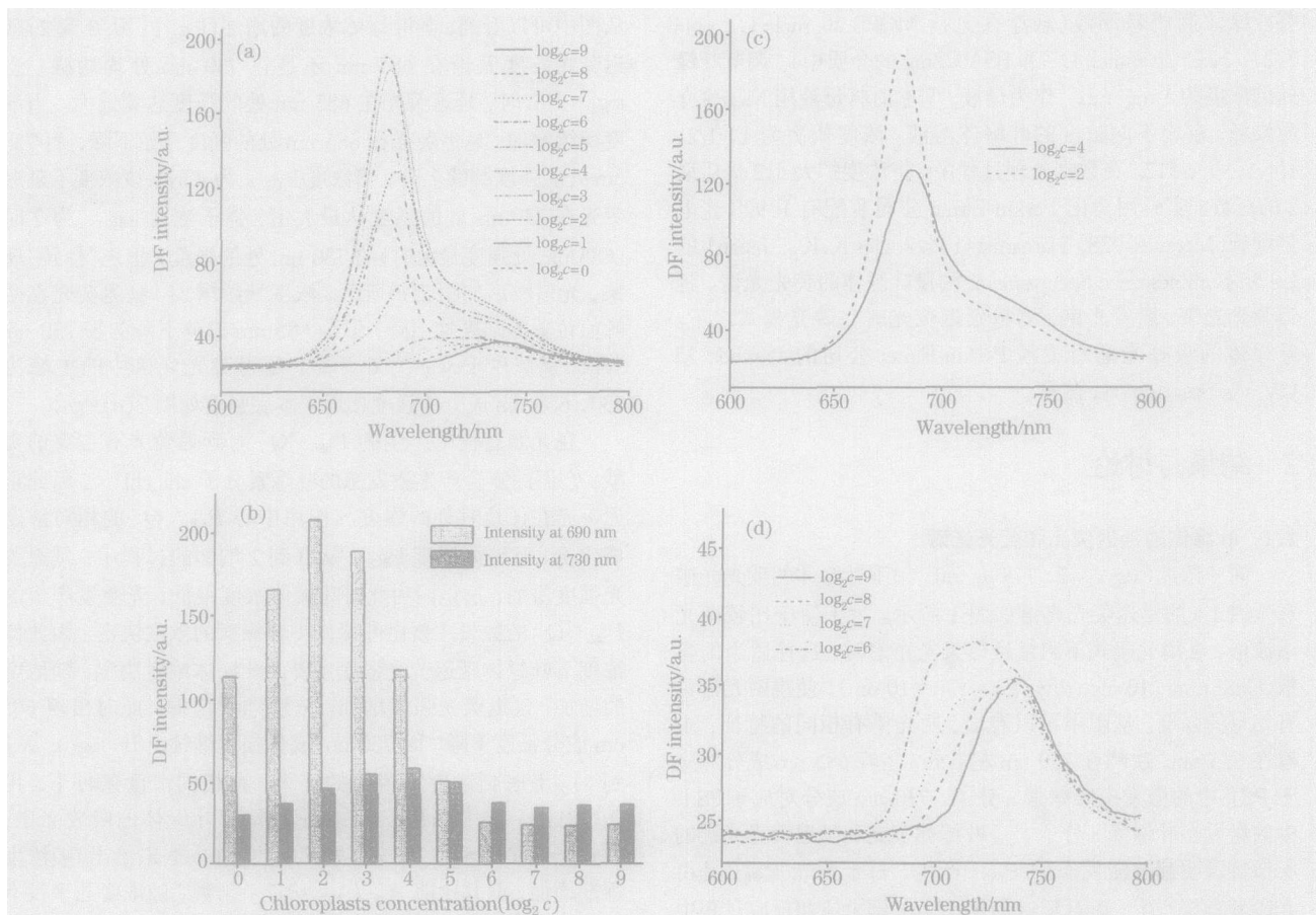
Fig. 2 (a) Effects of chloroplast concentration on delayed fluorescence spectra of isolated chloroplasts. (Excited by monochrome light (438 nm), slits: E_x = E_m = 5 nm, gate time = 1 ms) from bottom to top the chloroplast concentrations are in turn 1, 1/2, 1/4, 1/8, 1/16 ..... till 1/512 ( ) measured 1 s after the cessation of the excitation; (b) The value of DF intensity at 685/730 nm; (c) The delayed fluorescence spectra of isolated chloroplasts at \log_2 c = 2 and 4; (d) It showed the delayed fluorescence spectra when the concentration is continually increased.
