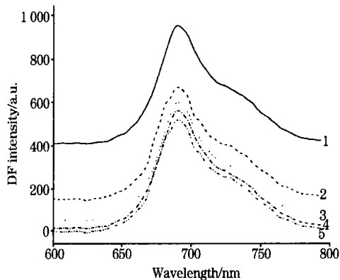
Fig. 6 Emission spectra of delayed fluorescence from isolated spinach chloroplasts ( \log_2 c = 2 , about 7.8 \mu\text{g} \cdot \text{mL}^{-1} ) measured at various times after the cessation of the excitation. (Excited by monochrome light (475 nm), slits: Ex = Em = 10 nm) from the top to bottom, the spectra measured after 1, 3, 5, 7 and 9 s, respectively 1, delayed 1 s; 2, delayed 3 s; 3, delayed 5 s; 4, delayed 7 s; 5, delayed 9 s
