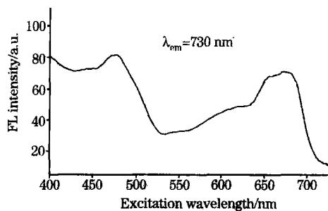
Fig. 4 The fluorescence excitation spectrum of spinach chloroplasts for 730 nm
