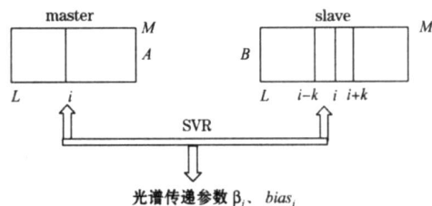
Fig 2 Computation of the transfer parameters in SVR procedure
