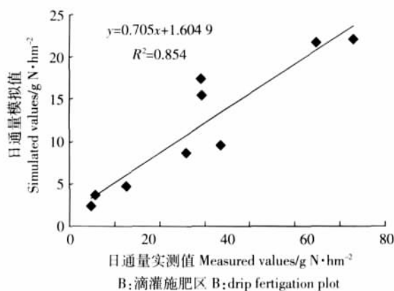
图 1 常规区和滴灌施肥区 N 2 O 日通量模拟值与实测值相关性 Figure 1 Correlation of simulated and measured values of N 2 O daily flux
