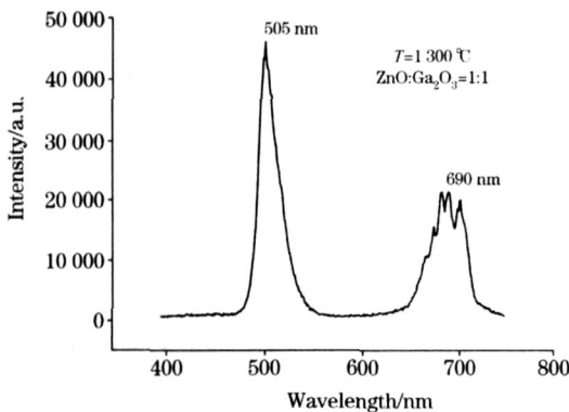
Fig 1 Afterglow spectrum of the ZnGa 2 O 4 phosphor excited by 254 nm T = 1 300 , ZnO : Ga 2 O 3 = 1 : 1
