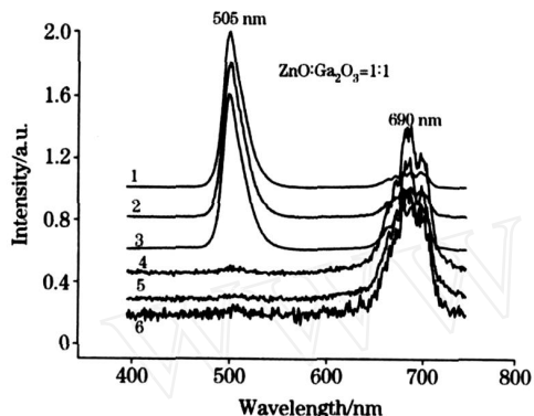
Fig. 5 Relative peak intensity of the samples prepared at different temperatures with the molar ratio ZnO : Ga 2 O 3 = 1 : 1
