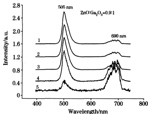
Fig. 7 Relative peak intensity of the samples prepared at different temperatures with the molar ratio ZnO : Ga 2 O 3 = 0.9 : 1
