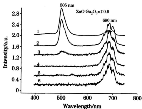
Fig. 6 Relative peak intensity of the samples prepared at different temperatures with the molar ratio ZnO : Ga 2 O 3 = 1 : 0.9
