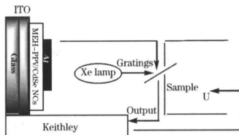
Fig 2 Schematics of nanocomposite device and electric circuit used for I - V and photocurrent action measurement
