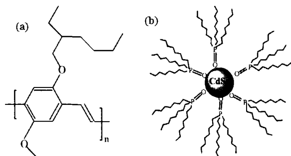
Fig 1 The structure of MEH-PPV (a) and TOPO capped CdSe nanocrystal (b)
