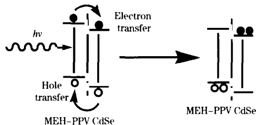
Fig 5 The schematic illustration of the exciton and charge transfer and exciton dissociation in the composite device
