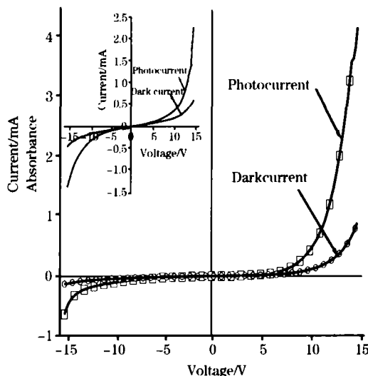
Fig 3 Current voltage curve for a device containing 60( wt%) CdSe and 40( wt%) MEH-PPV in the dark and under illumination at 500 nm. The inset shows the current voltage curve for a pure MEH-PPV device
