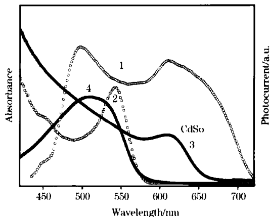
Fig 4 Photocurrent action spectra of a pure MEH-PPV device and a nanocomposite device. Absorption spectra of MEH-PPV and CdSe nanocrystals are also shown
