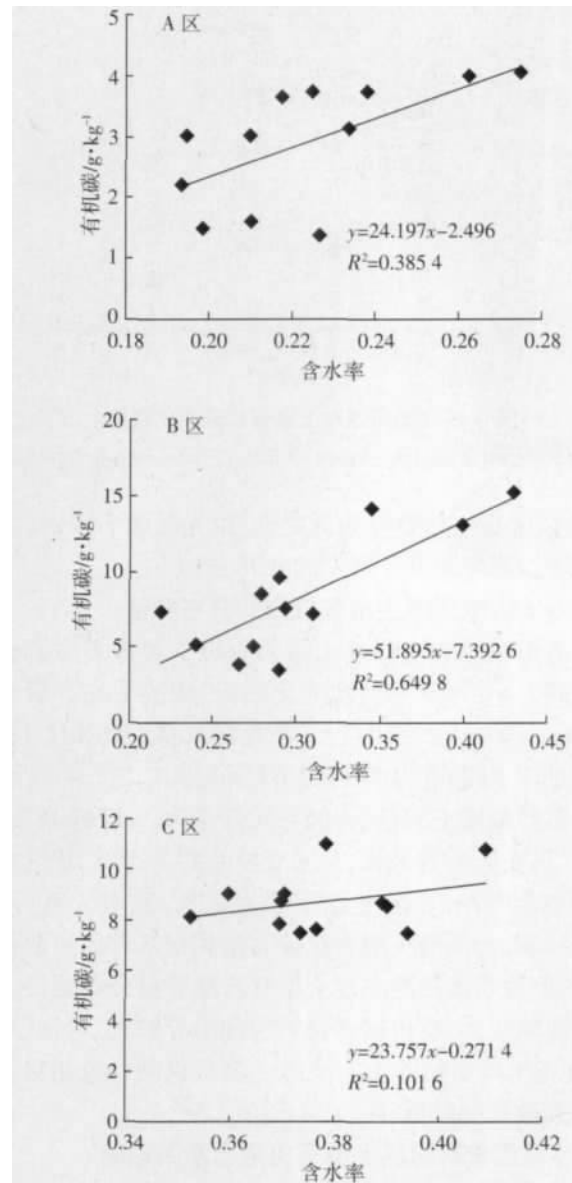
图7 不同区域湿地土壤含水率与有机碳的关系 Figure 7 Relationship of moisture content and organic carbon in different zone
