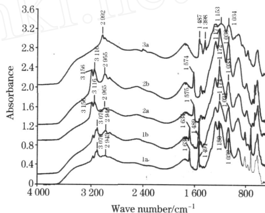
Fig 2 IR spectra of five ionic liquids
