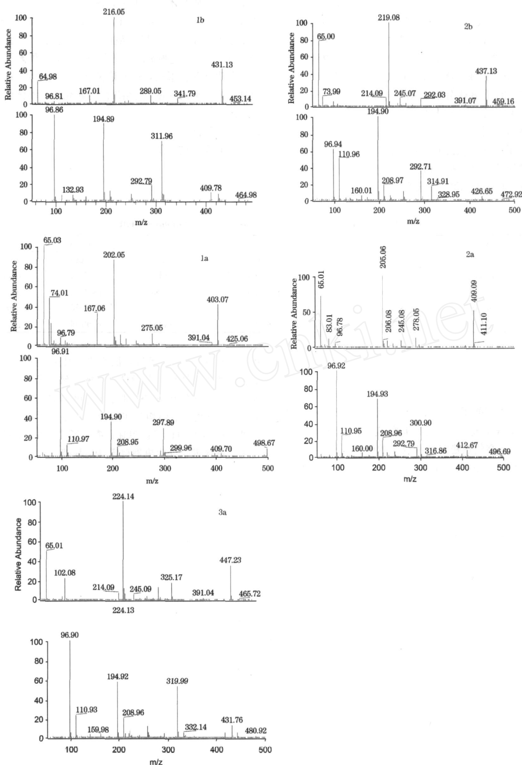
Fig 3 Electrospray ionization mass spectra (ESFMS) of five ionic liquids
