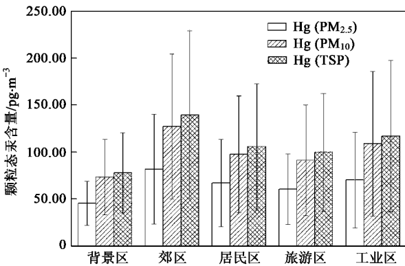
图 2 采样点颗粒态汞年平均浓度 Fig. 2 Annual average concentration of atmospheric particulate mercury in different sites
