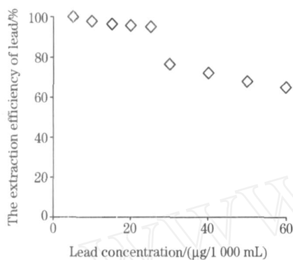
Fig 2 Effect of amount of lead concentration on the extraction efficiencies
