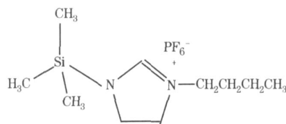
Fig 1 1-butyl-3-trimethylsilylimidazolium hexafluorophosphate
