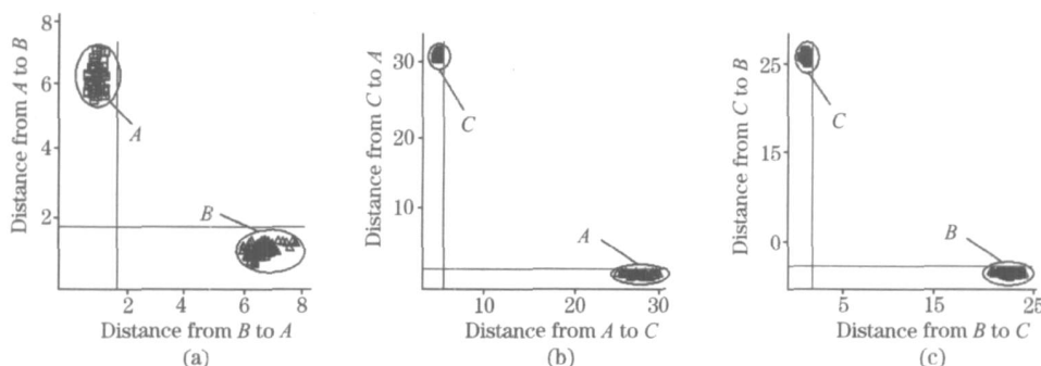
Fig 2 Class plot of A, B and C from classification of principal component analysis-Mahalanobis distance
