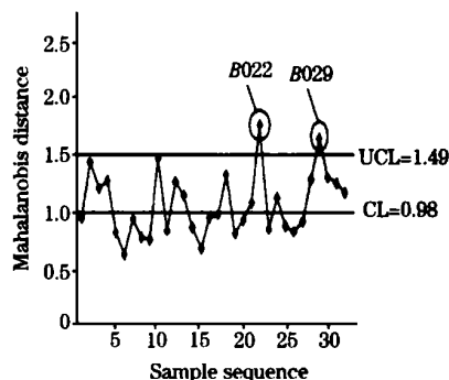
Fig 3 3 \sigma -control plot of Mahalanobis distance for B class
