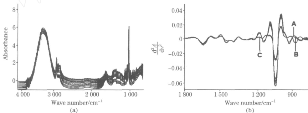
Fig 1 FTIR-ATR spectra of tobacco flavour (a) and their 2nd derivative spectra(b)
